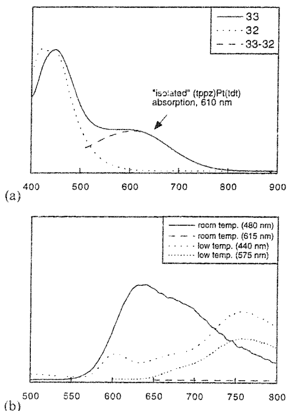
Fig. 7. Absorption and emission spectra of [(\text{dbbpy})_2\text{Ru}(\text{tppz})\text{Pt}(\text{Cl}_2)](\text{PF}_6)_2 ( 32 ) and [(\text{dbbpy})_2\text{Ru}(\text{tppz})\text{Pt}(\text{idt})](\text{PF}_6)_2 ( 33 ). (a) UV-visible absorption in \text{CH}_2\text{Cl}_2 and (b) emission spectra of 33 at room temperature in \text{CH}_2\text{Cl}_2 and at 77 K in butyronitrile glass.
