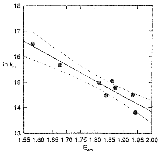
Fig. 3. Plot of \ln(k_{\text{nr}}) versus E_{\text{em}} for the series of complexes 3–10 showing an energy gap law correlation. The solid line corresponds to a linear least squares fit and the dotted lines denote 95% confidence limits.
