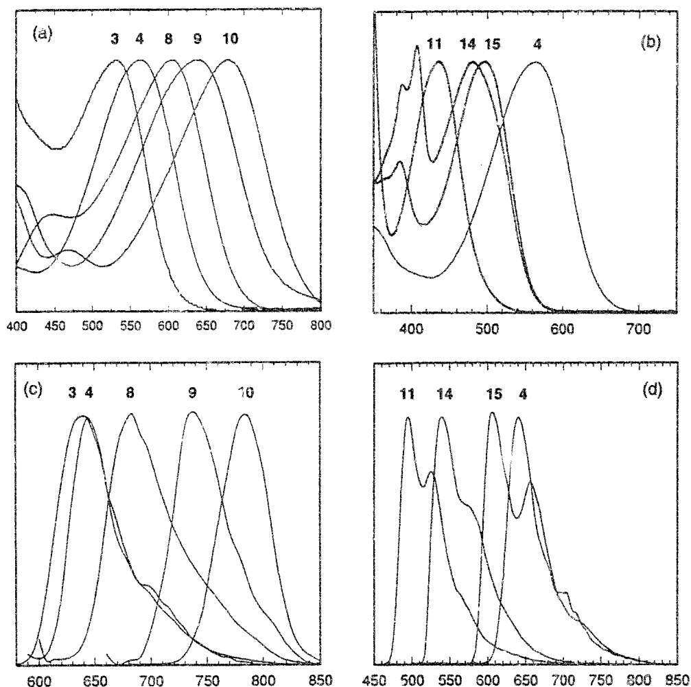
Fig. 1. Normalized absorption and emission bands for Pt(dimmine)(dithiolate) complexes: (a) solvatochromic absorption bands for Pt(diimine)(tdt) complexes in dichloromethane; (b) solvatochromic absorption bands for Pt(dbbpy)(dithiolate) complexes in dichloromethane; (c) emission bands for Pt(diimine)(tdt) complexes in frozen butyronitrile at 77 K; (d) emission bands for Pt(dbbpy)(dithiolate) complexes in frozen butyronitrile at 77 K.
