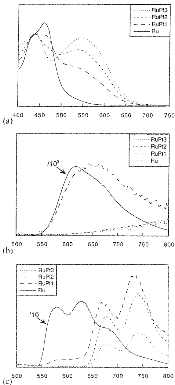
Fig. 6. Absorption and emission spectra of [(\text{dbbpy})_{3-n}\text{Ru}(\text{dpca})\text{Pt}(\text{dbbpy})_n](\text{PF}_6)_2 (RuPtn, n = 1-3 , 28–30) and [\text{Ru}(\text{dbbpy})_3](\text{PF}_6)_2 (Ru). (a) UV-visible absorption in \text{CH}_2\text{Cl}_2 ; (b) room temperature emission in \text{CH}_2\text{Cl}_2 ; (c) low temperature emission in butyronitrile glass.
